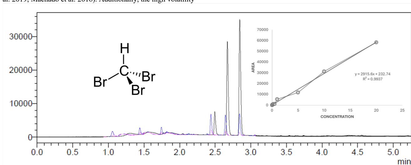
Figure 4: Overlay of chromatograms for standard bromoform (black), Sample A (blue), and Sample B (pink).
