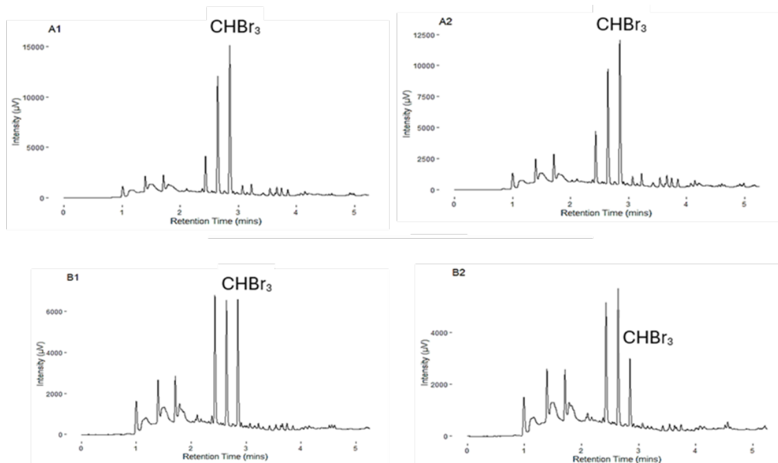
Figure 5: Chromatograms of Specimen A and B, illustrating the elution of bromoform with a retention time of 2.85 minutes.
